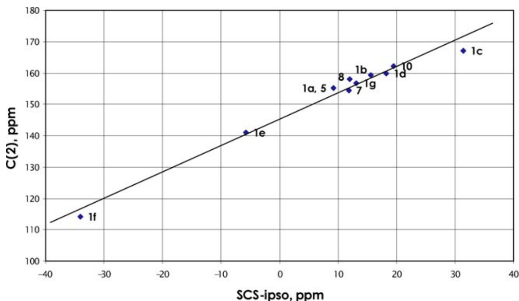
FIGURE 1 Plot of chemical shifts ( \delta ) of carbon 2 in iodofurazans vs SCS_i values for monosubstituted benzenes.
